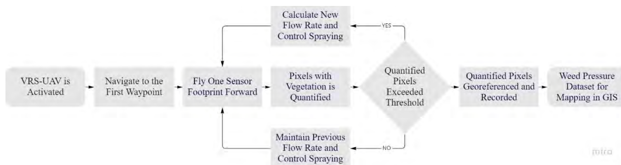
Figure 1. The flowchart of proposed image-based UAV variable rate spraying subsystem.
